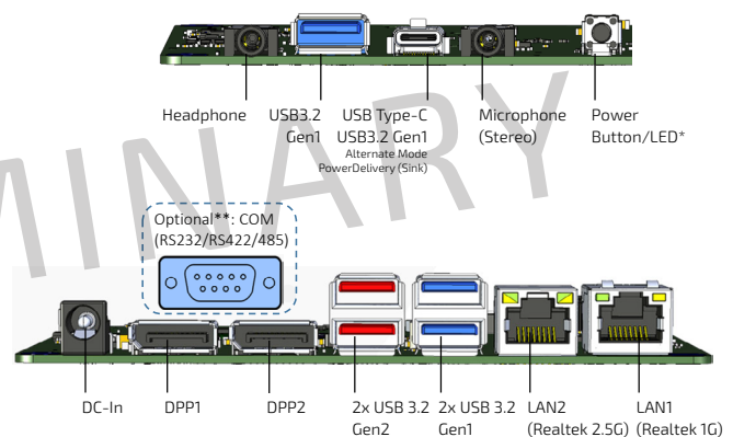
*) Prepared for SMARTCASE™ S501 chassis kit **) Via optional COM port cable. Breakout feature SC501 chassis rear I/O
